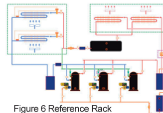
Figure 6 Reference Rack system diagram with DTC valve
