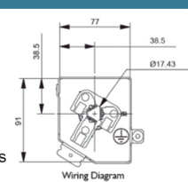
Figure 8 Motor terminal connections
