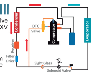
Figure 3 Reference LT system diagram with DTC Valve
