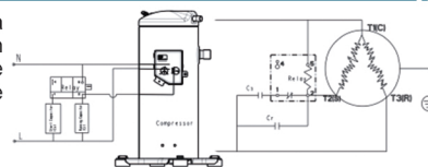
Figure 5 Wiring Diagram of start kits
